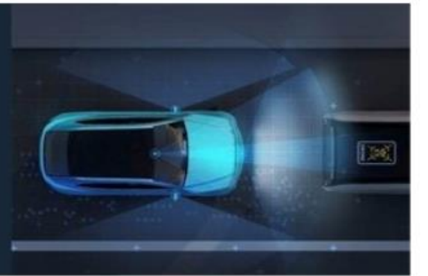
Obstacle Avoidance
